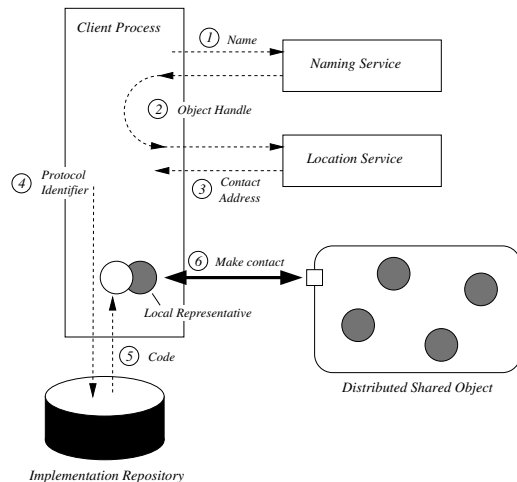
Figure 1. Binding to a GlobeDoc object
